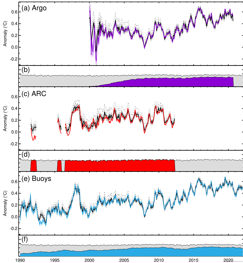
Figure 7: From [14]. Comparison to instrumentally homogeneous data sets. (a) global average SST anomalies from Argo (purple) and HadSST.4.0.1.0 (black and grey shading). The dotted line shows a global average calculated from unadjusted data. All comparisons are colocated. (b) coverage of HadSST.4.0.1.0 (grey) and coverage of the Argo data (purple). (c) and (d) as for (a) and (b) but for ARC data. (e) and (f) as for (a) and (b) but for drifting buoy data.
