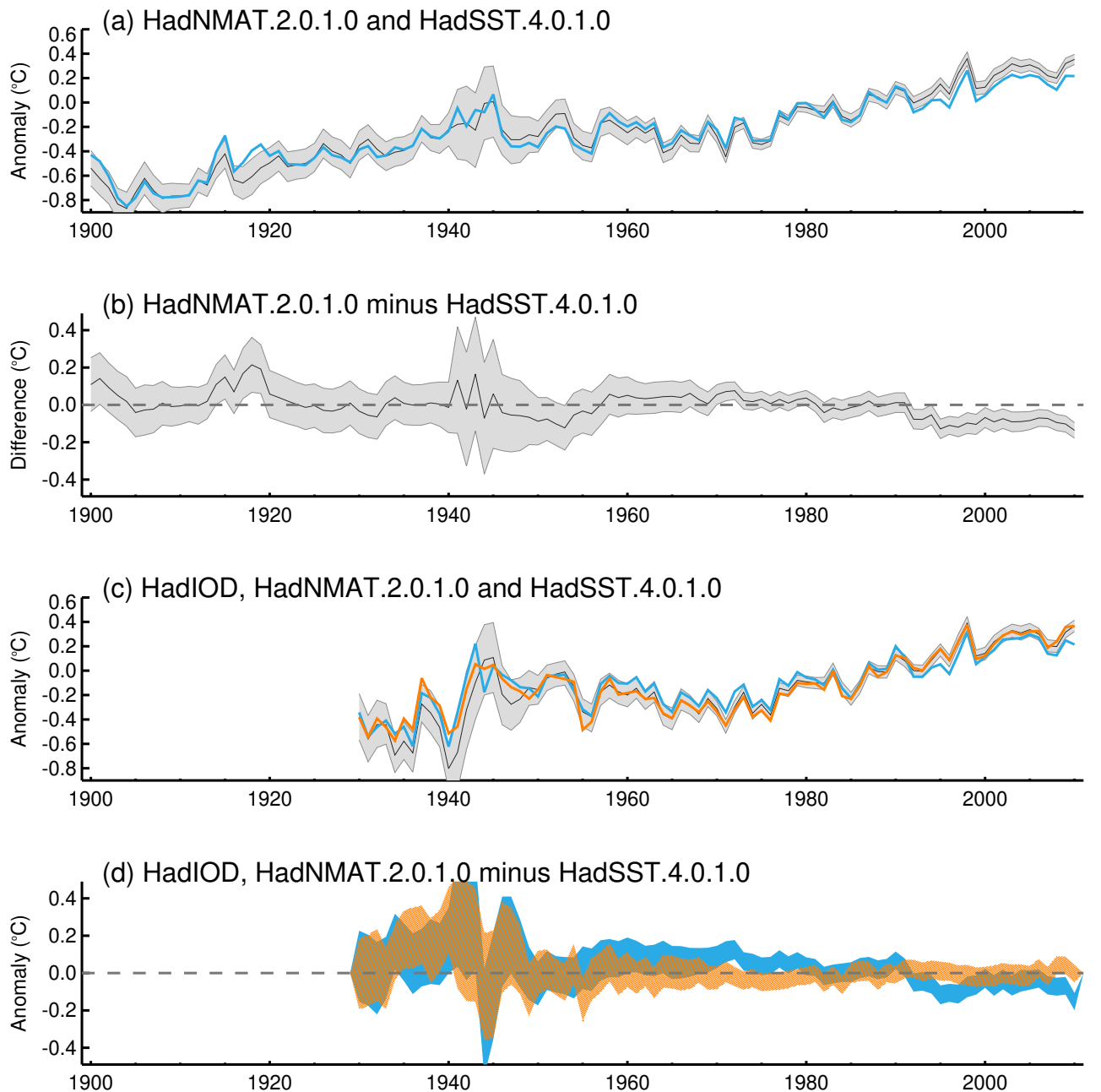
Figure 6: From [14]. (a) Collocated global annual average NMAT anomalies (°C) 1900-2010 offset by 0.15°C (blue, relative to 1961-1990) and global annual average SST anomalies from HadSST.4.0.1.0 (black is central estimate and grey shading indicates 95% uncertainty range). (b) Offset NMAT anomalies minus SST anomalies with combined 95% uncertainty range (taking into account the bias errors from the HadSST.4.0.1.0 ensemble, and measurement and sampling errors in the SST). The dashed line indicates zero difference. (c) Collocated global annual average offset NMAT anomalies (blue), global annual average near-surface water temperature from HadIOD excluding Argo (orange) and SST (black is central estimate and grey shading again indicates 95% uncertainty range). (d) Difference between HadIOD and HadSST.4.0.1.0 (orange) and NMAT and HadSST.4.0.1.0 (blue). The shaded area indicates the 95% uncertainty range..
