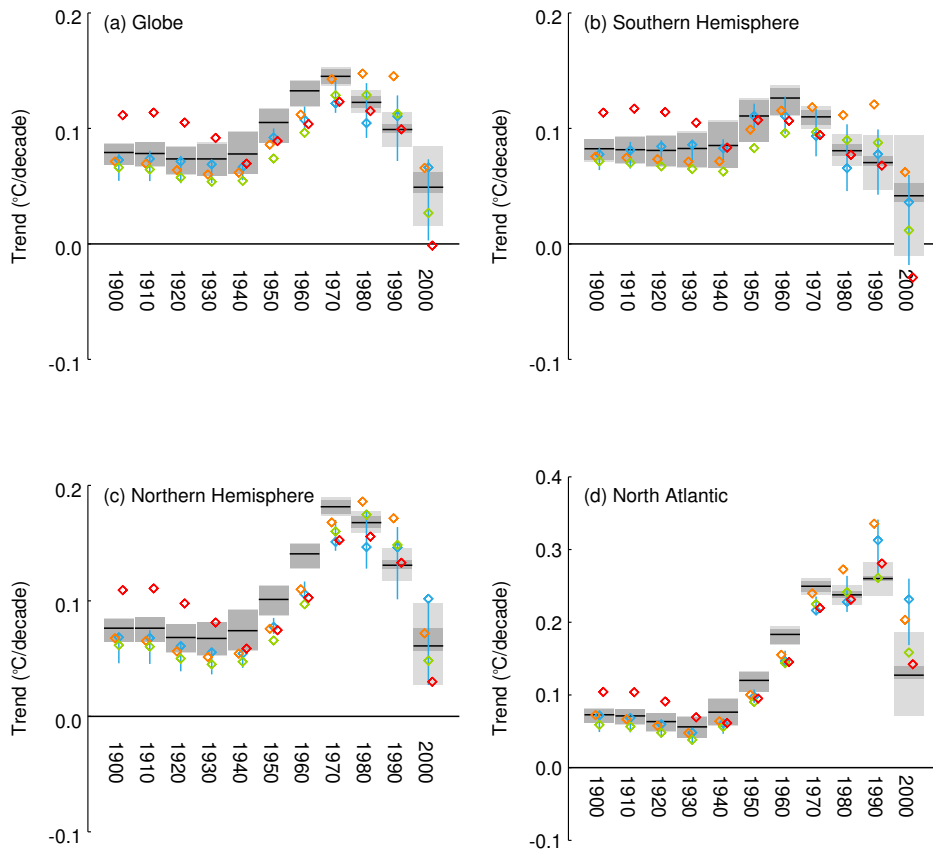
Figure 5: Updated from [14]. Global and regional average SST anomaly trends to 2012. Median trends from HadSST.4.0.1.0 are indicated by a black horizontal line and the grey shading indicates median and 95% uncertainty range including effects from measurement, sampling and bias-adjustment errors. The bias-adjustment uncertainty range is shown in darker grey; ERSSTv5 (blue), the lozenge is the operational version and the vertical line is the 95% ensemble range from the 1000-member ERSSTv4 ensemble); COBE-SST-2 (orange); HadSST.3.1.1.0 (green); and unadjusted SSTs (red).
