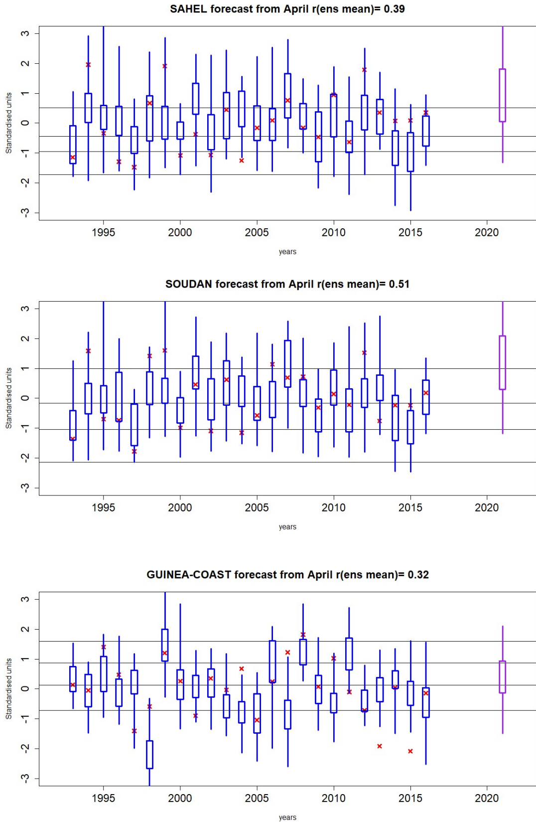
Figure 1.2: GloSea6 ensemble predictions for July-August-September 2021 (purple box-and-whisker far right) and corresponding retrospective forecasts (blue box-and-whisker) and observed rainfall (red crosses) for each year 1993-2016 and for the 3 North African regions. Solid horizontal lines are the quintile boundaries scaled as in Part 2.
