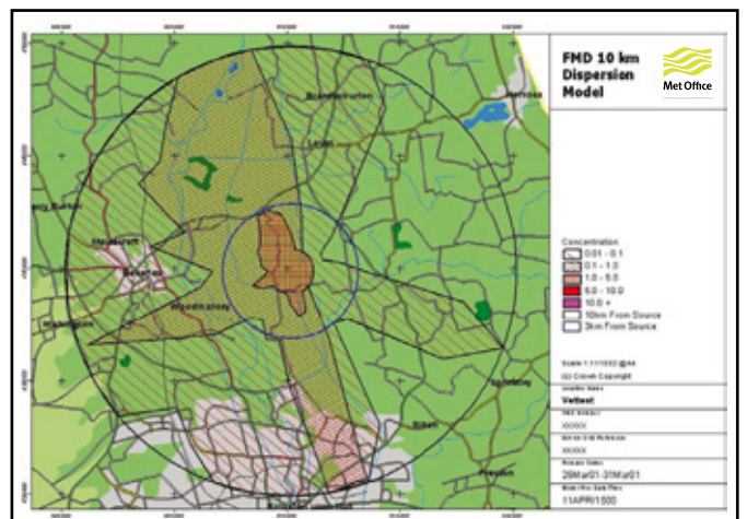
Figure 11 - An example of how NAME is used to predict the spread of Foot and Mouth disease.
