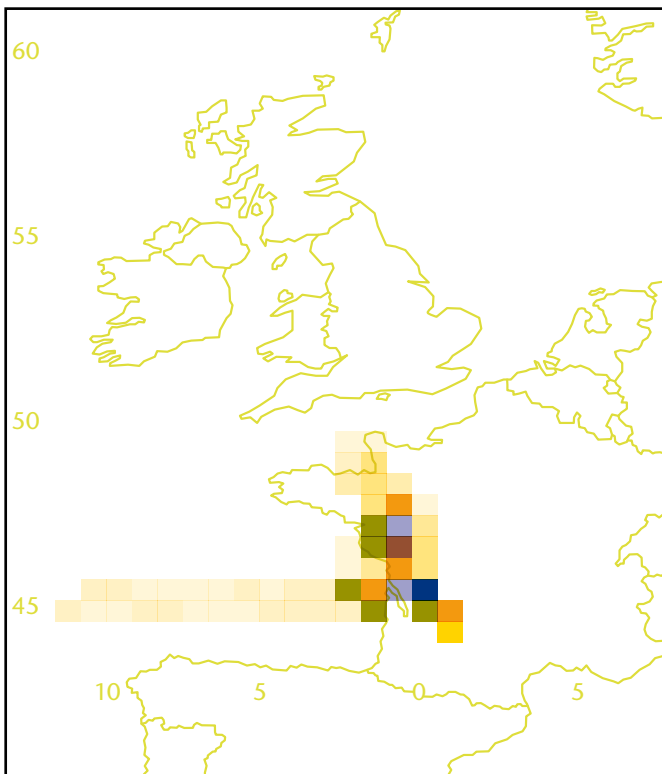
Figure 14 - Source identification derived from running NAME backwards in time.
