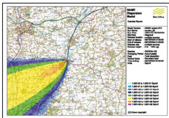
Figure 8 - An example of NAME output.
