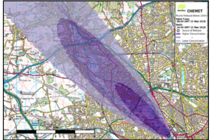
Figure 9 - An example of a CHEMET 'Plume below 100 metres' map originating from a site close to Cardiff City Centre on 15 March 2018.
