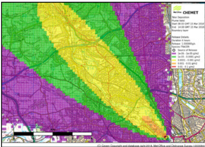
Figure 10 - A sample CHEMET Pro deposition map produced for a location in Cardiff using the real time weather conditions on 15 March 2018.
