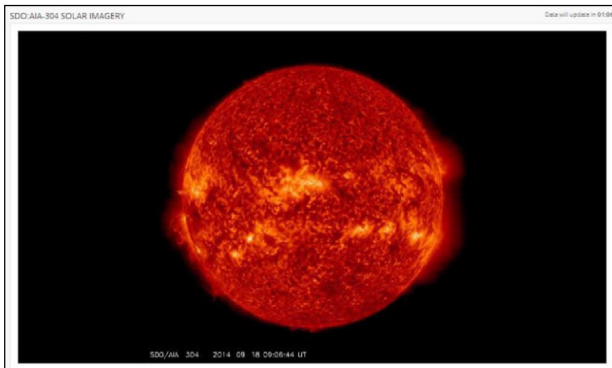
Figure 16 - An example of the solar imagery used in the Met Office Space Weather Operations Centre (MOSWOC).
