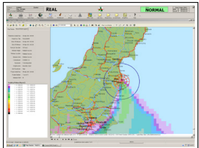
Figure 13 - An example of plume prediction from the Fukushima incident in 2011, as displayed on the RIMNET system.
