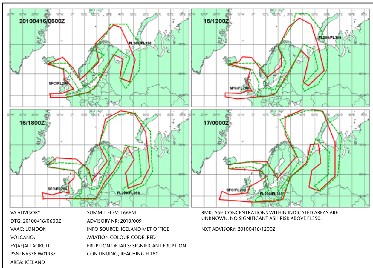
Figure 15 - Volcanic Ash Advisory issued during the Eyjafjallajökull eruption in April 2010.
