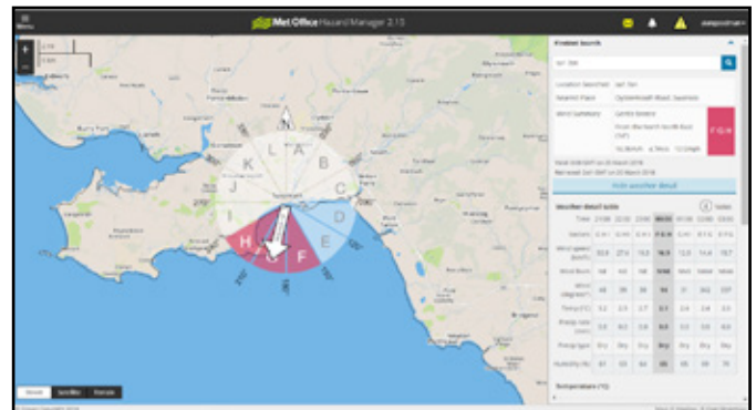
Figure 7 - FireMet data display from 20 March 2018, using Swansea City Centre as a reference point.
